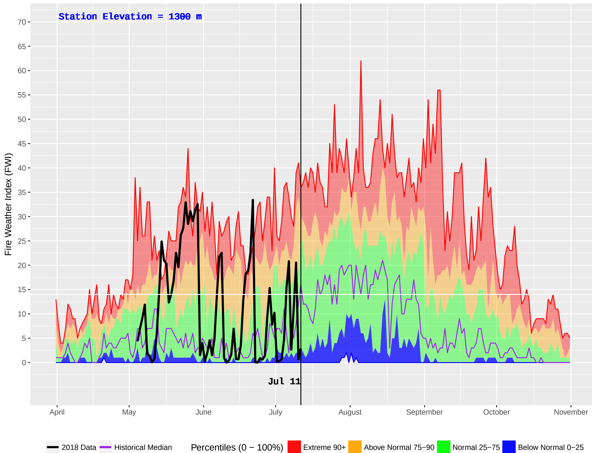
MARION (367) : Historical (1994–2016) and Current (2018) Noon Fire Weather Index (FWI)
