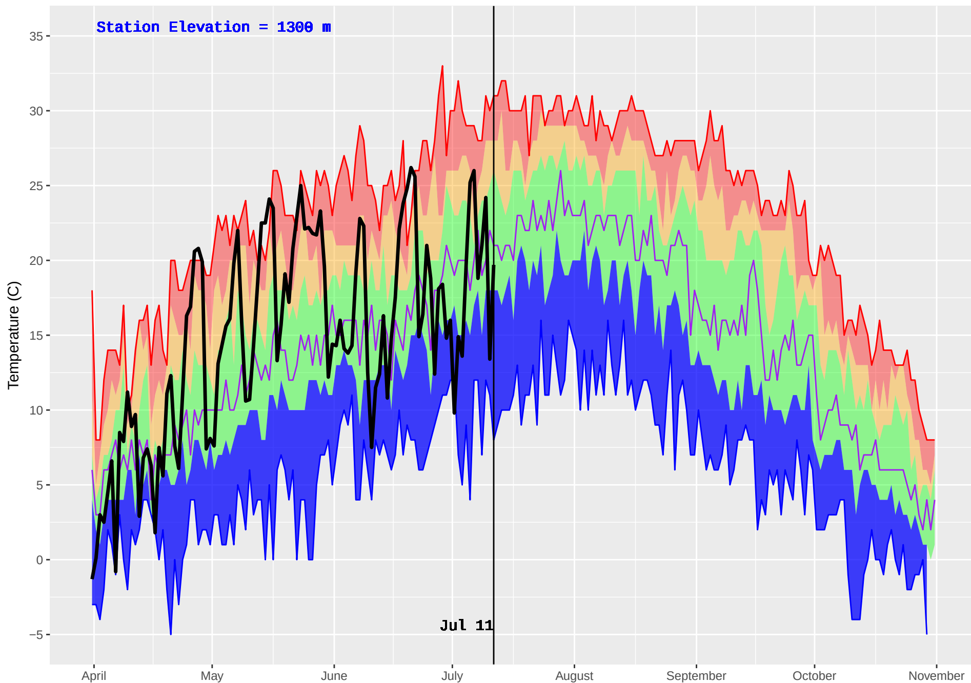
MARION (367) : Historical (1994–2016) and Current (2018) Noon Temperature
