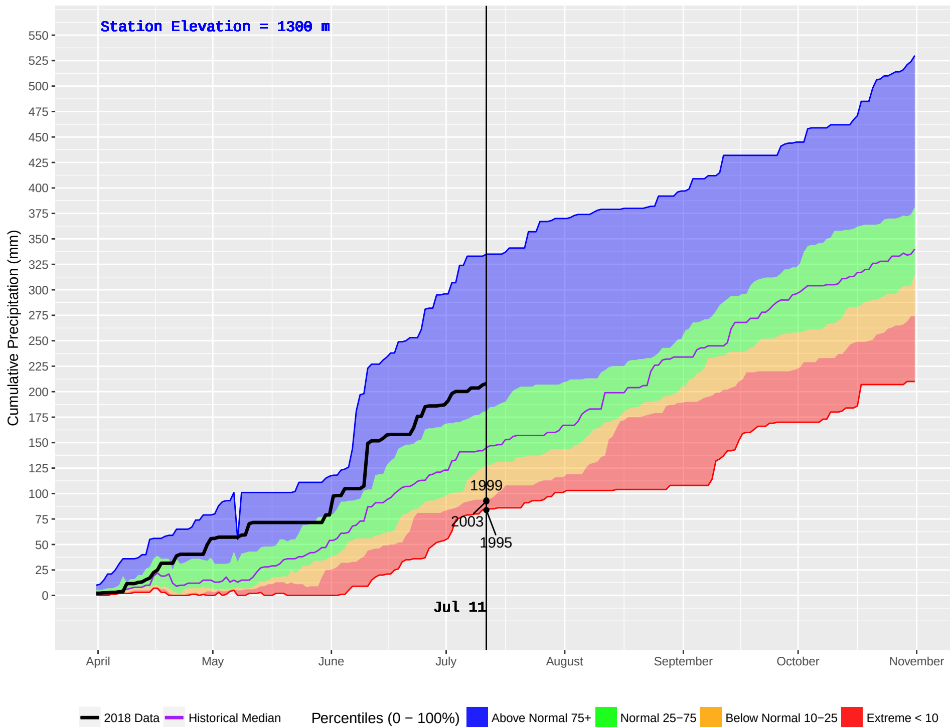
MARION (367) : Historical (1994–2016) and Current (2018) Noon Cumulative Precipitation
