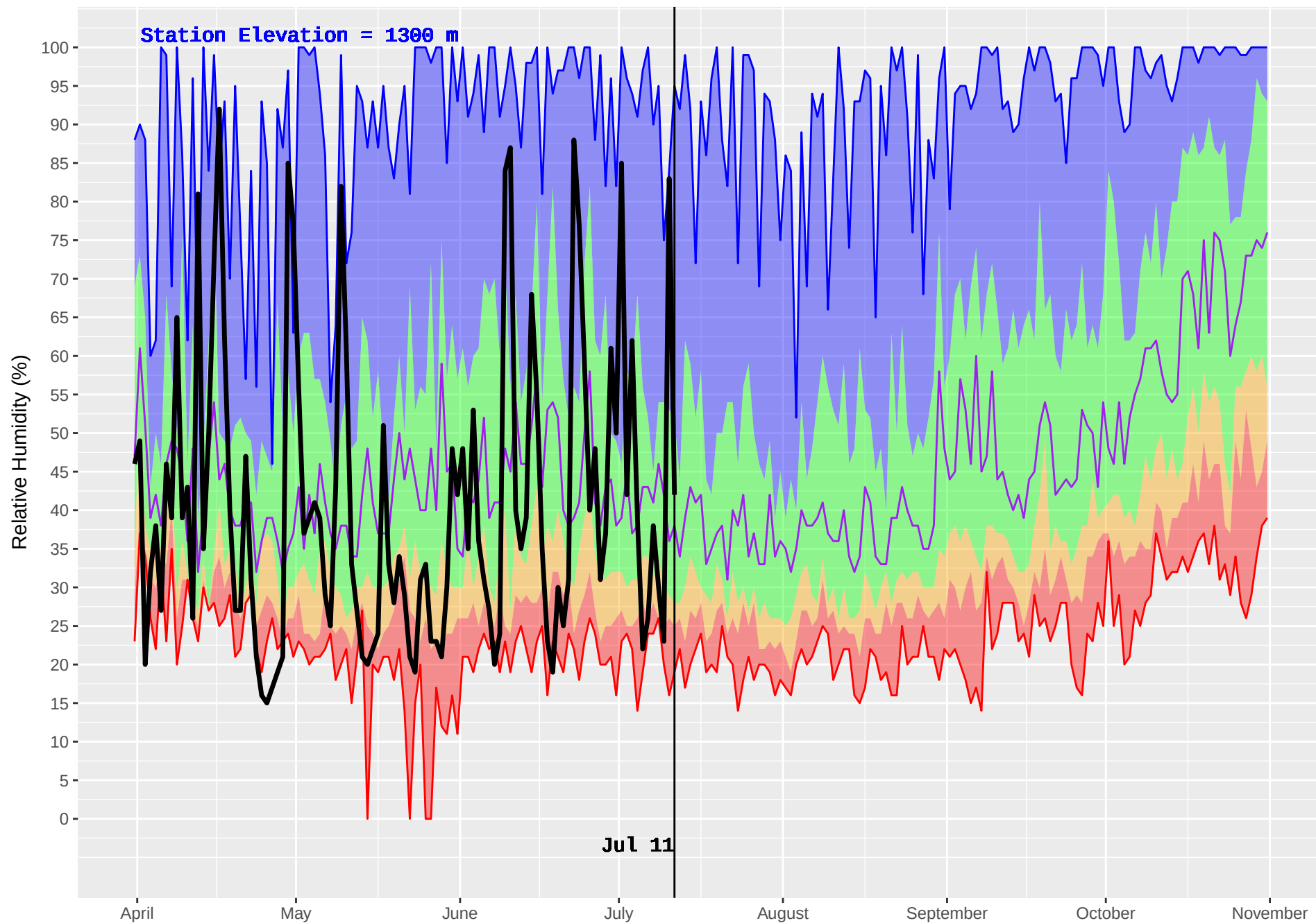
MARION (367) : Historical (1994–2016) and Current (2018) Noon Relative Humidity
