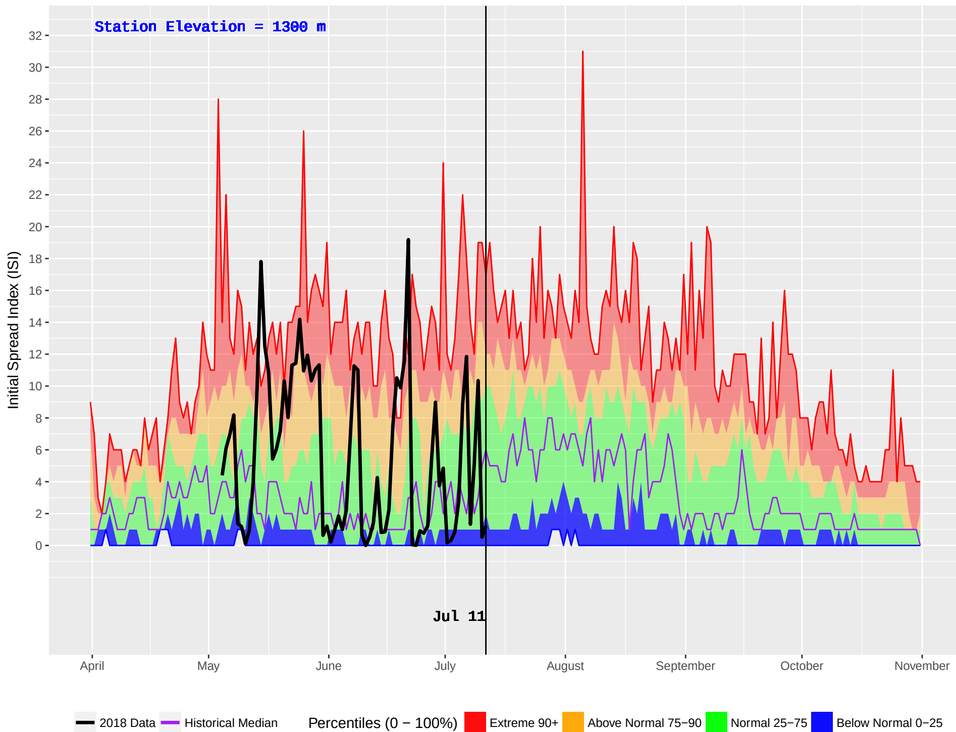
MARION (367) : Historical (1994–2016) and Current (2018) Noon Initial Spread Index (ISI)
