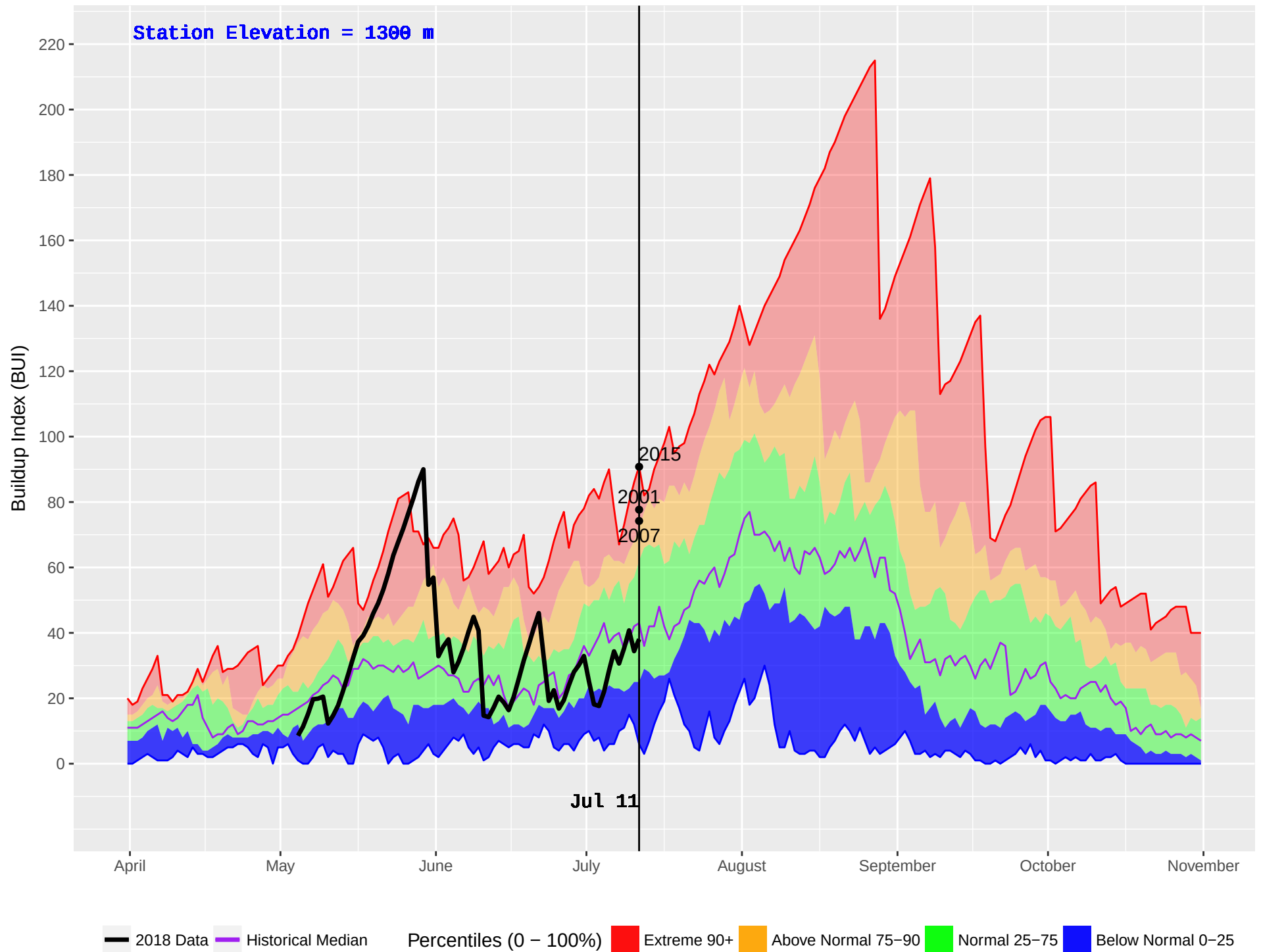
MARION (367) : Historical (1994–2016) and Current (2018) Noon Buildup Index (BUI)
