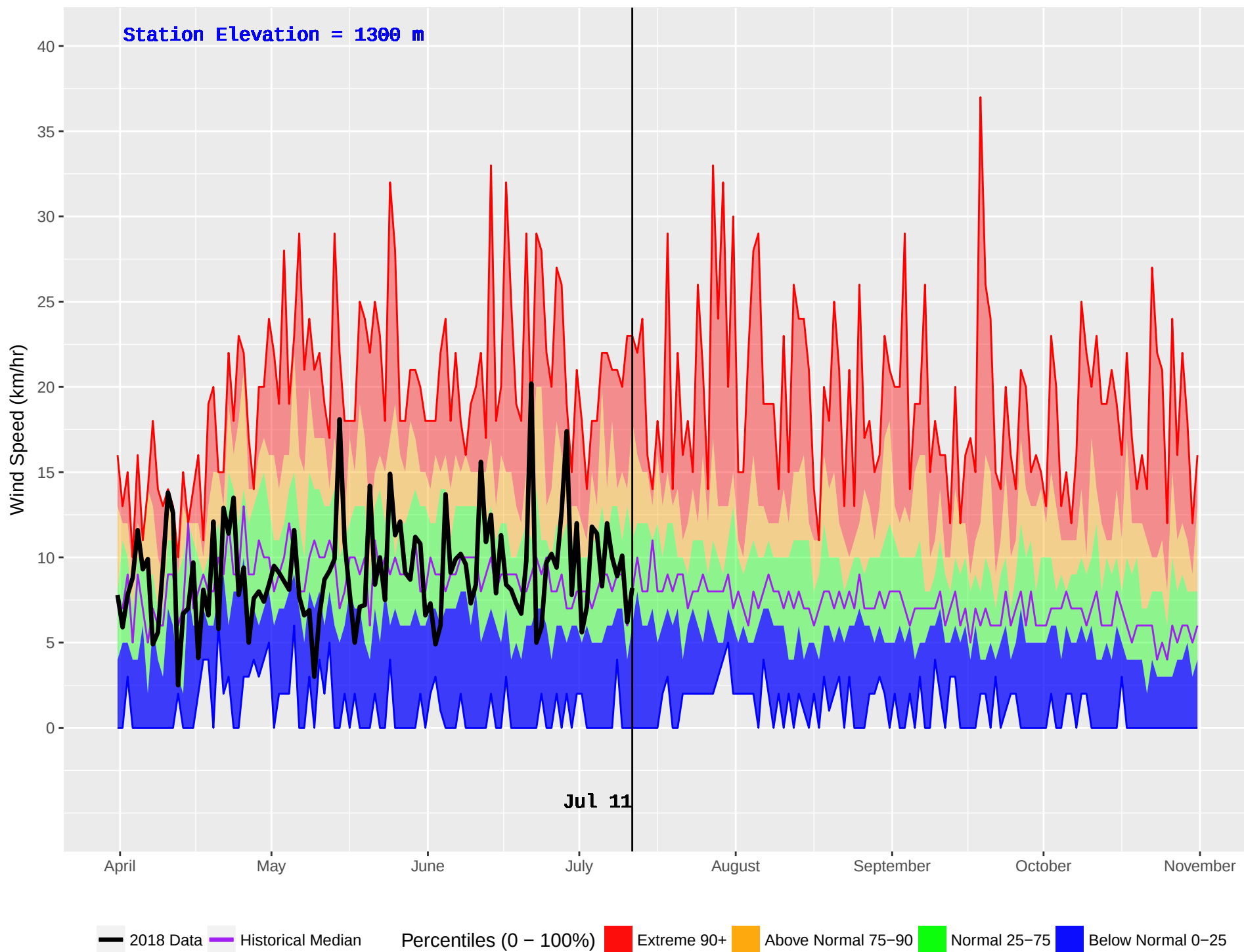
MARION (367) : Historical (1994–2016) and Current (2018) Noon Wind Speed
