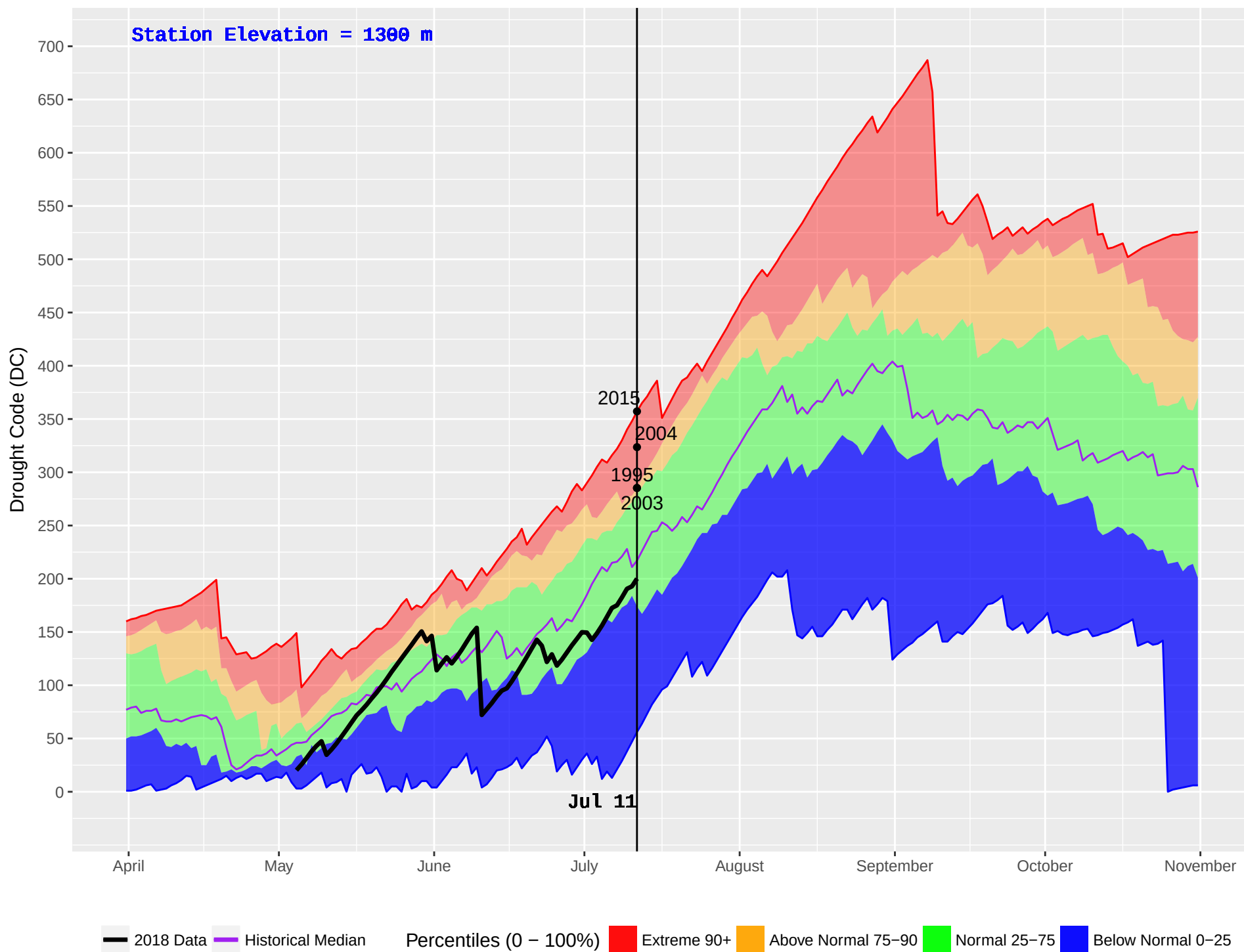
MARION (367) : Historical (1994–2016) and Current (2018) Noon Drought Code (DC)
